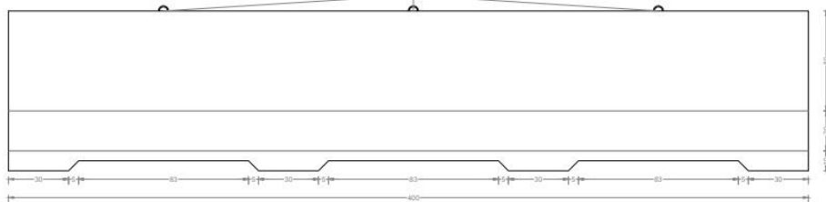
VISTA FRONTAL L = 4 m
