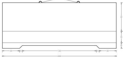
VISTA FRONTAL L = 2 m
