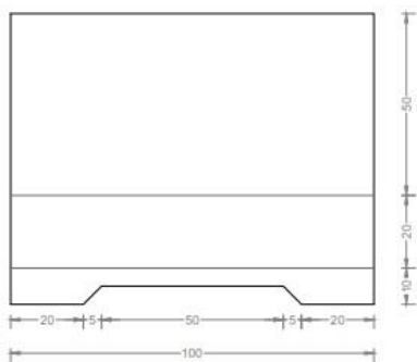
VISTA FRONTAL L = 1 m
